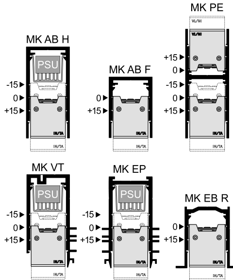
Figure 3: Latch positions depending on profile type
